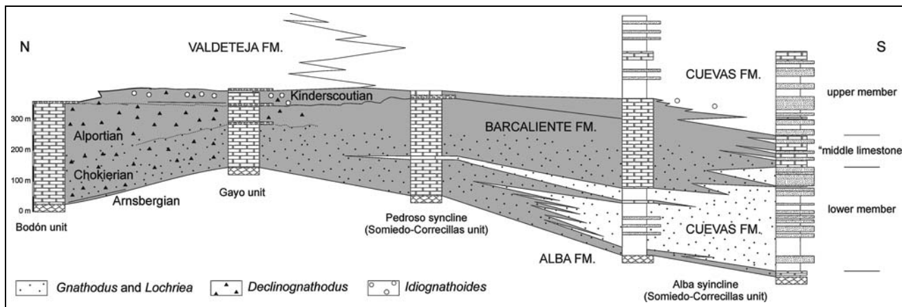
Fig. 2 - Correlation scheme between different composite stratigraphic sections of the Barcaliente Formation at Bernesga Valley (data after Wagner et al. 1971, Reuther 1977, Alonso et al. 1991, and Menéndez-Álvarez 1991). Location is in Fig. 1 and horizontal scale is free. Vertical and horizontal distributions of some conodont genera are outlined.
