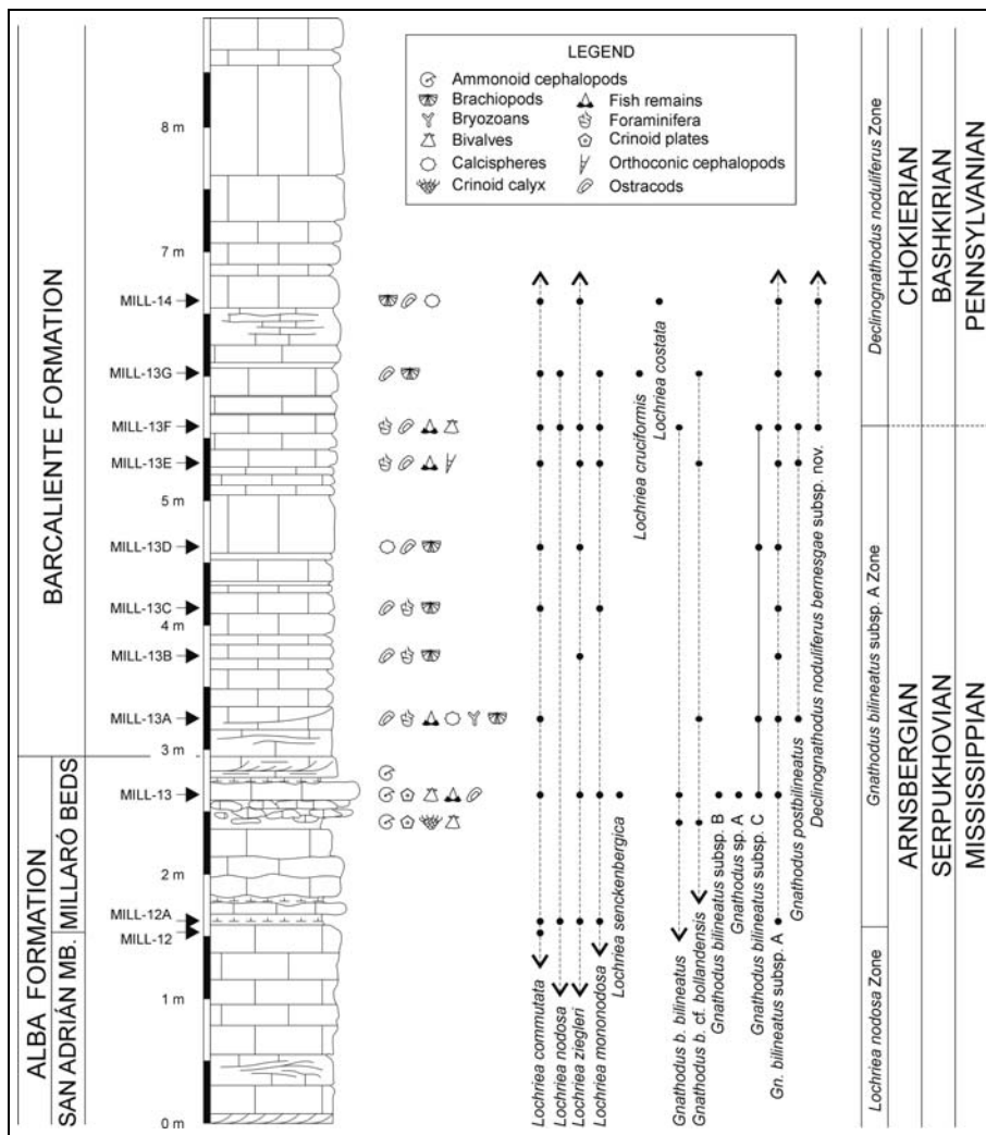
Fig. 3 - Detailed stratigraphic section and conodont content of the Millaró Beds and lowermost part of the Barcaliente Formation at the Millaró section (Cantabrian Zone).
