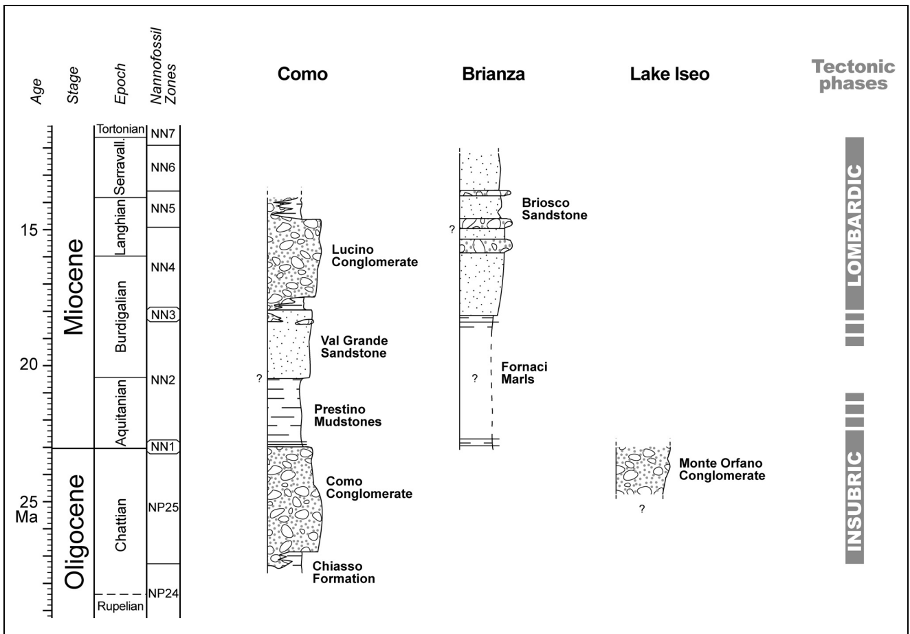
Fig. 4 - Correlation of the GLG units in Lombardy. The westernmost outcrop area of the GLG (Varese) was not considered, due to the absence of calcareous nannoplankton biostratigraphy. Time scale from Gradstein et al. (2005); nomenclature and timing of alpine tectonic “phases” after Schumacher et al. (1997).
