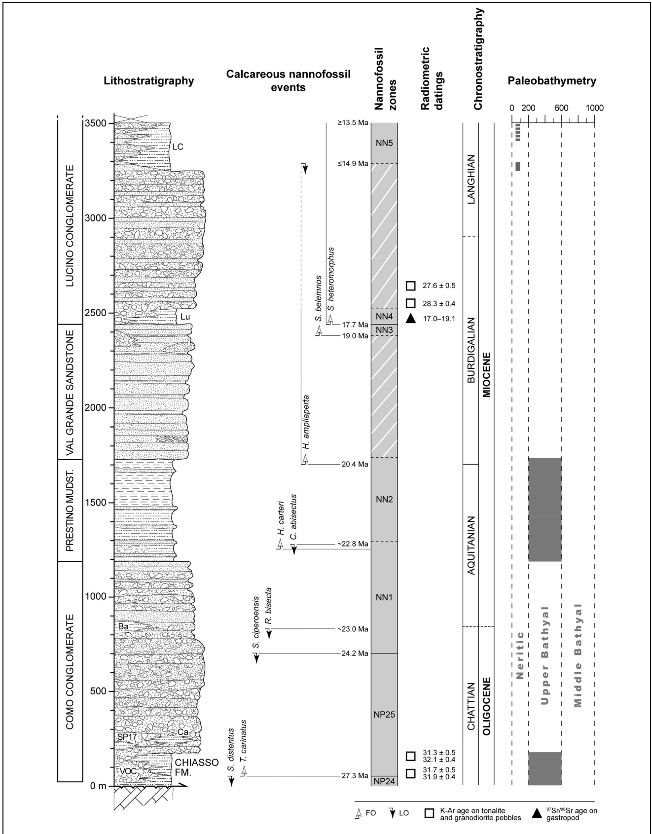
Fig. 3 - Composite stratigraphic section of the Gonfolite Lombarda Group with indication of, from left to right, lithostratigraphic units, calcareous nannofossil biostratigraphic events, radiometric data from Giger & Hurford (1989) and Bernoulli et al. (1993), chronostratigraphic interpretation, and paleobathymetry. Important mudstone levels intercalated in the Como Conglomerate are documented by samples GLG 24-25 (SP17), GLG 26-29 (Ca), and GLG 31-33 (Ba). VOC: Villa Olmo Conglomerate; Ca: Castello; Ba: Baradello; Lu: Lucinasco Mudstones; LC: Lurate Caccivio Mudstones. Cumulative stratigraphic thickness from Napolitano (1985) and new stratigraphic calculations; nannofossil events and numerical ages from Berggren et al. (1995), Gradstein et al. (2005), and Raffi et al. (2006).
