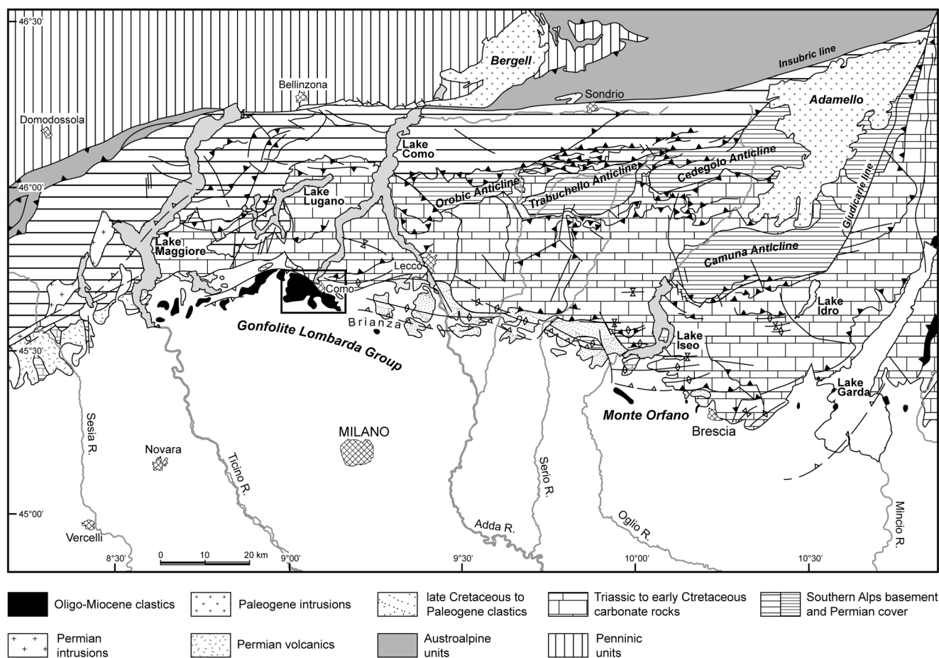
Fig. 1 - Geologic sketch map of the Southern Alps (modified from Schumacher et al. 1997), with the study area (box).
