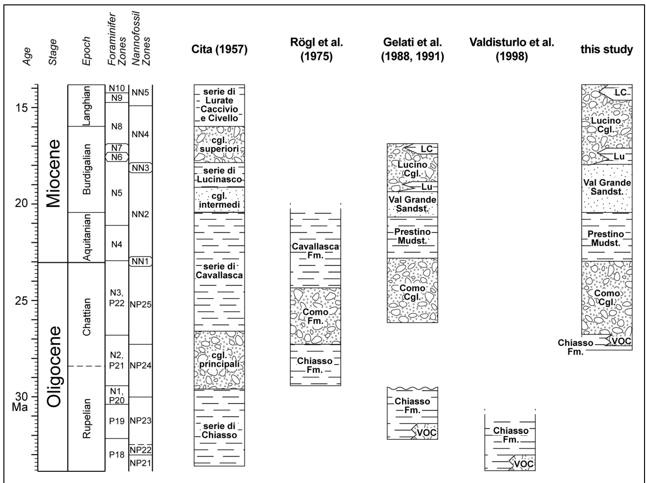
Fig. 2 - Synopsis of the GLG litho- and biostratigraphy according to selected studies across a 50-years time span. Open upward columns refer to studies only dealing with a partial sector of the GLG. VOC = Villa Olmo Conglomerate; Lu: Lucinasco Mudstones; LC: Lurate Caccivio Mudstones. Time scale is from Gradstein et al. (2005).
