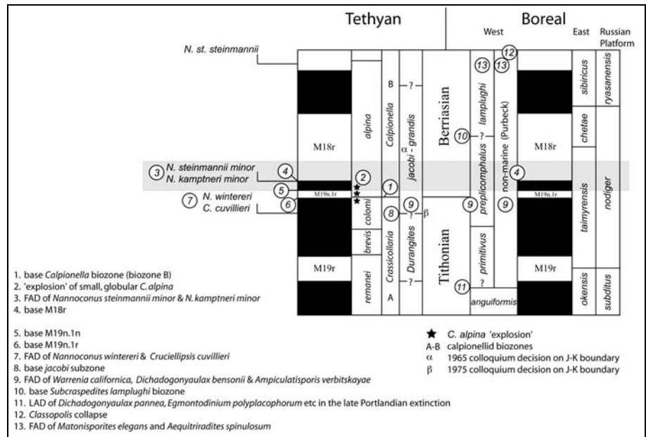
Fig. 1 - Markers under examination as potentially useful in defining the Jurassic/Cretaceous boundary interval.
