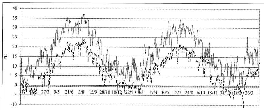
Fig. 1 - Minimum and maximum temperature in the whole period of study. (Data from Stezzano - Bergamo province, provided by Ersaf - Ente Regionale Servizi Agricoltura e Foreste).
