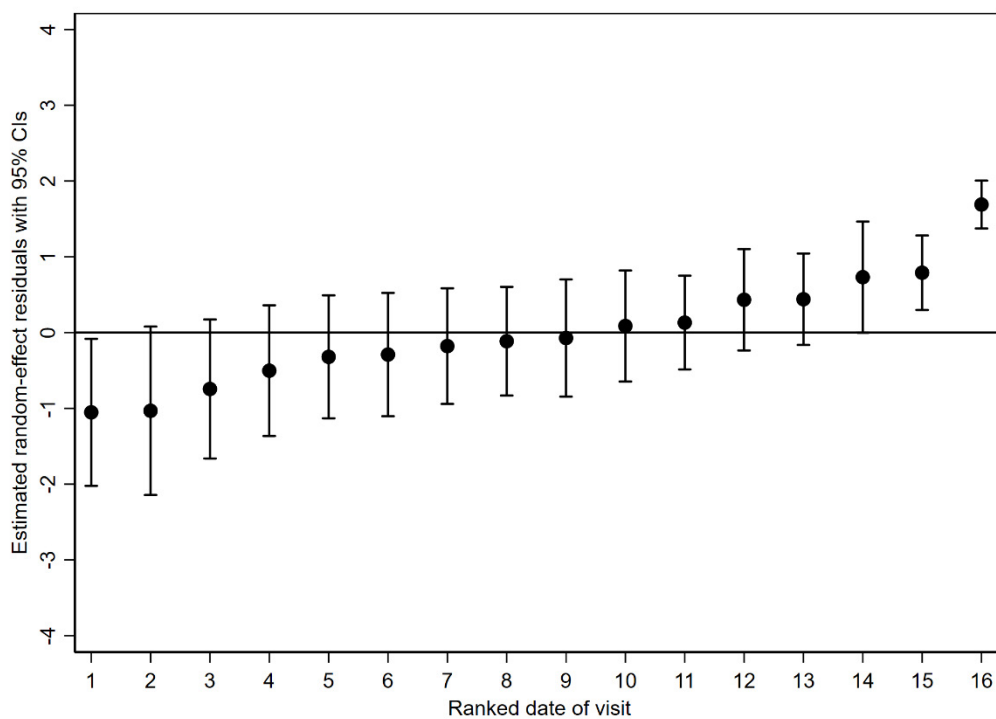
FIGURE 2. Caterpillar plot showing estimated 2nd level variances
